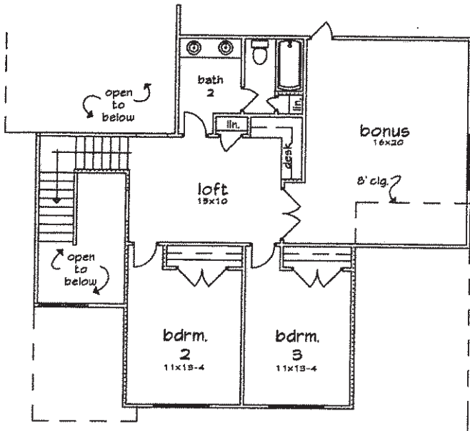
2ND LEVEL FLOOR PLAN
