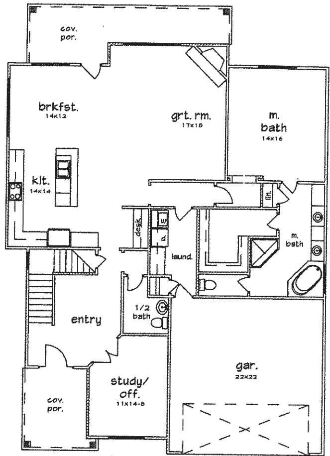
1ST LEVEL FLOOR PLAN 2400-395-3117
